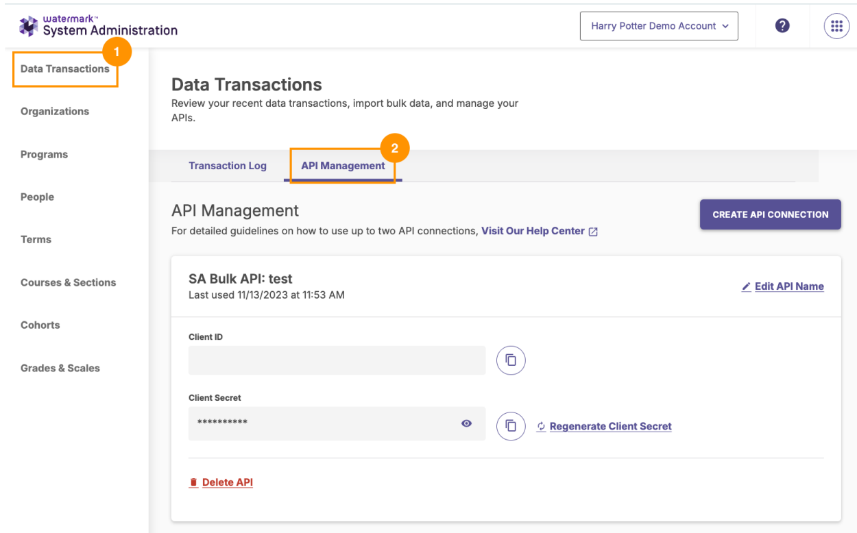
Figure 2: Obtain new credentials by clicking on the “Create API Connection” button.
